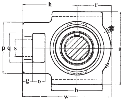
UCT 200 Type Normal Duty - setscrew
